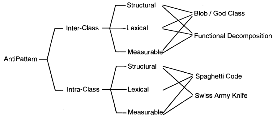
FIG. 3.3 – Classification des anti-patrons.
