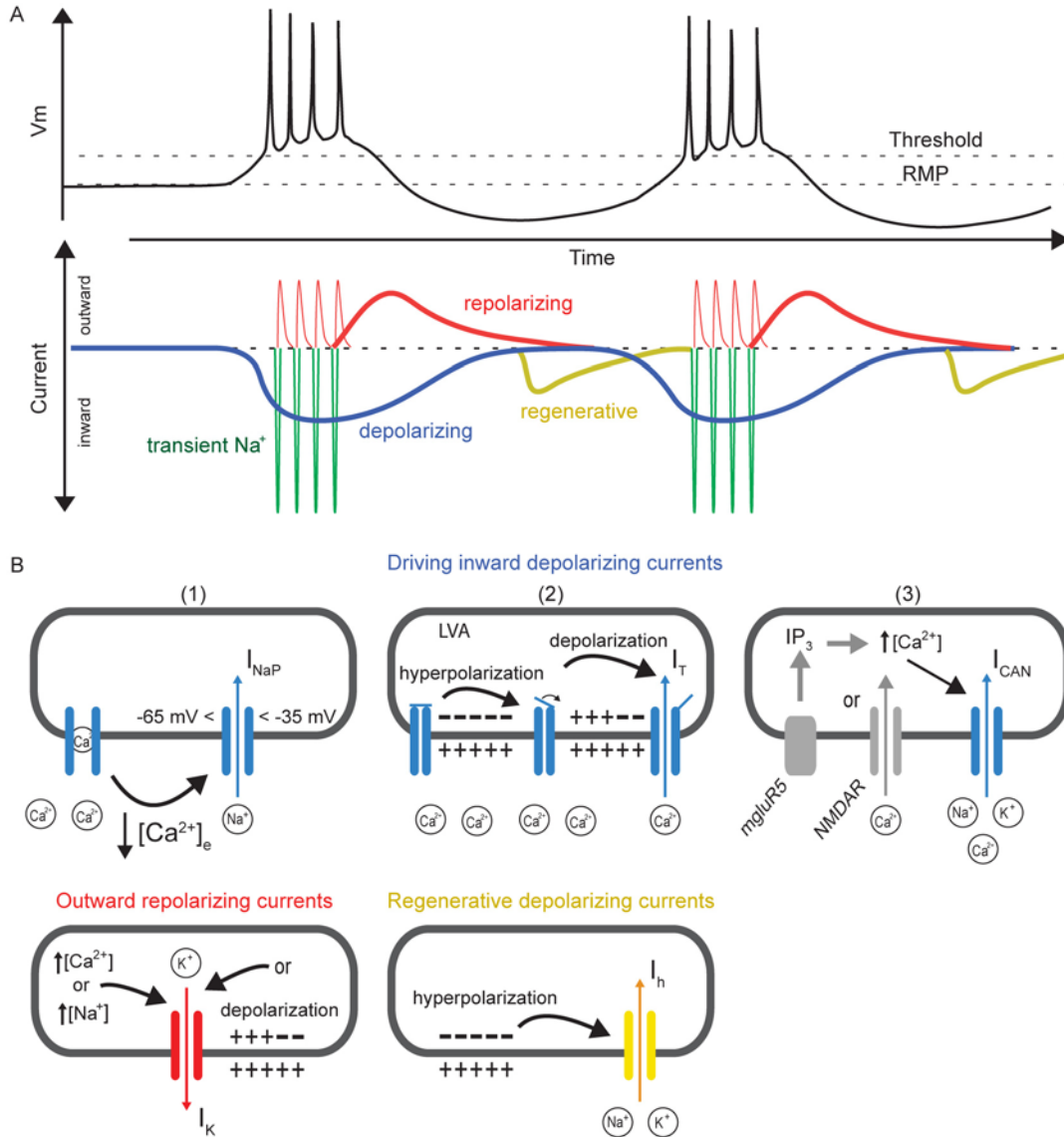
Figure 1. Ionic currents underlying repetitive bursting. A , Representation of two bursts (top) and the sequence of activation of the underlying ionic currents (bottom). Repetitive bursting generally relies on activation of a conductance that produces a sustained depolarization or plateau (blue) and “drives” the membrane potential from the resting level (RMP) to the threshold for activation of transient sodium currents (dark green) responsible for action potentials. Voltage-gated potassium channels (red) repolarize the membrane after each of these action potentials while other potassium channels activated by Ca^{2+} and Na^+ entering the cell during depolarization and firing slowly repolarize the membrane often to a level below RMP. In many instances, the hyperpolarization triggers activation of I_h which enables regeneration of the cycle by depolarizing the membrane potential and allowing for reactivation of the driving current. B , Top: Different channels responsible for driving the depolarizing plateaus supporting bursting and the conditions required for their activation. Bottom: Channels required for repolarization and burst termination (red; left) and for regenerating the depolarizing drive (yellow; right).
