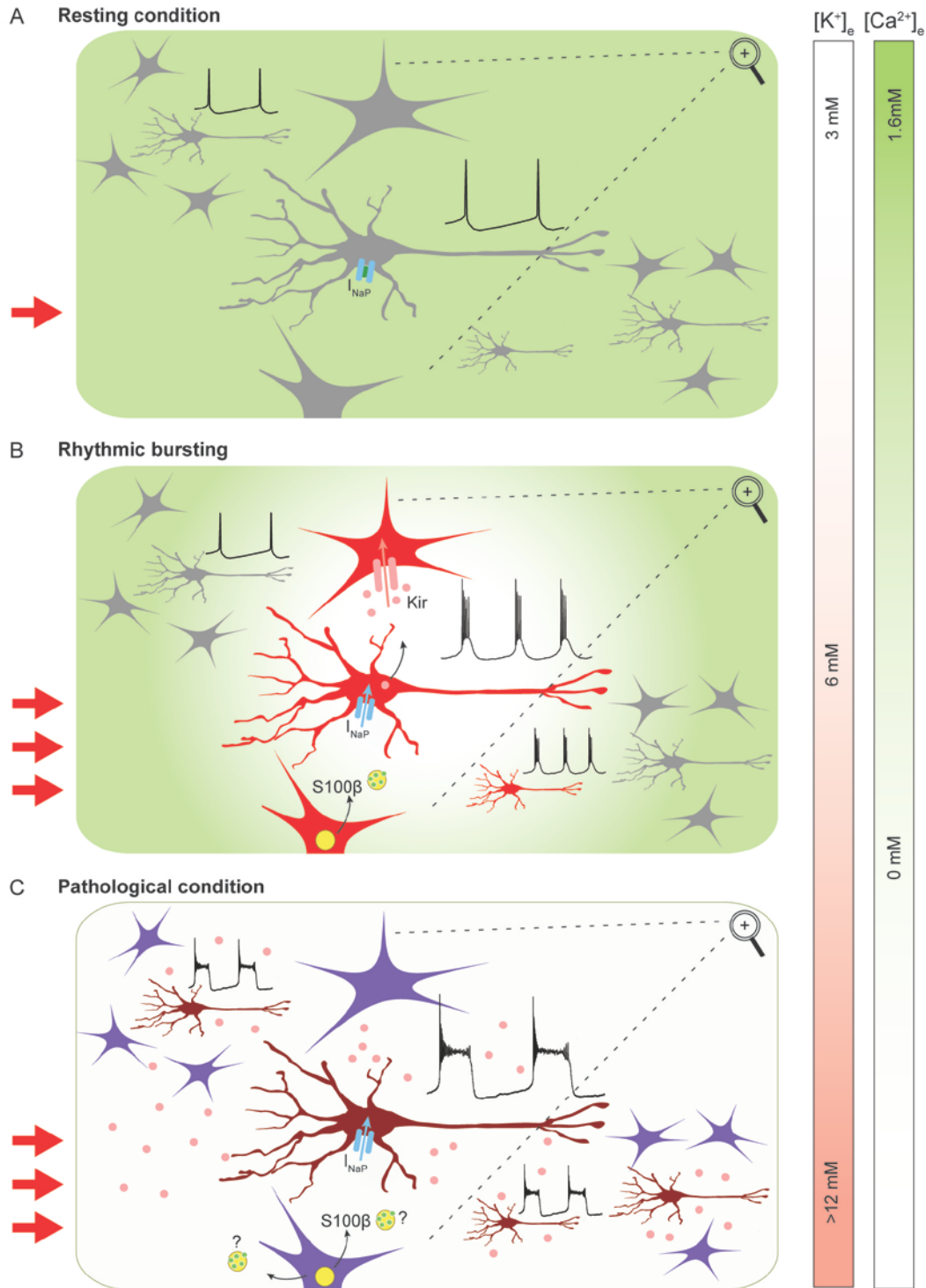
Figure 4. A general model for rhythmogenesis in CPGs. A , Under resting conditions, glutamatergic inputs are low (red arrow), astrocytes (grey) are at resting activity levels, [Ca^{2+}]_e is elevated and [K^+]_e is low. The I_{NaP} channels are obstructed by calcium (green dot) and neurons fire tonically. B , As the glutamatergic inputs increase, [K^+]_e (pink dots) rises, astrocytes get activated (red), release S100 \beta (yellow) and initiate spatial buffering through Kir channels. Protein S100 \beta chelates calcium and causes [Ca^{2+}]_e to drop. As a consequence, I_{NaP} channels are freed and drive bursting in neurons (red). The bursting population is limited to the extent of coupled astrocytes forming a syncytium. C , Under pathological conditions, astrocytes (purple) fail to initiate spatial buffering in the presence of intense neuronal activity, leading to an accumulation of potassium (pink dots) and spread of excitation and depolarization block among neurons. The level of S100 \beta in the extracellular space may increase and further lead to neuronal hyperexcitability by decreasing [Ca^{2+}]_e .
