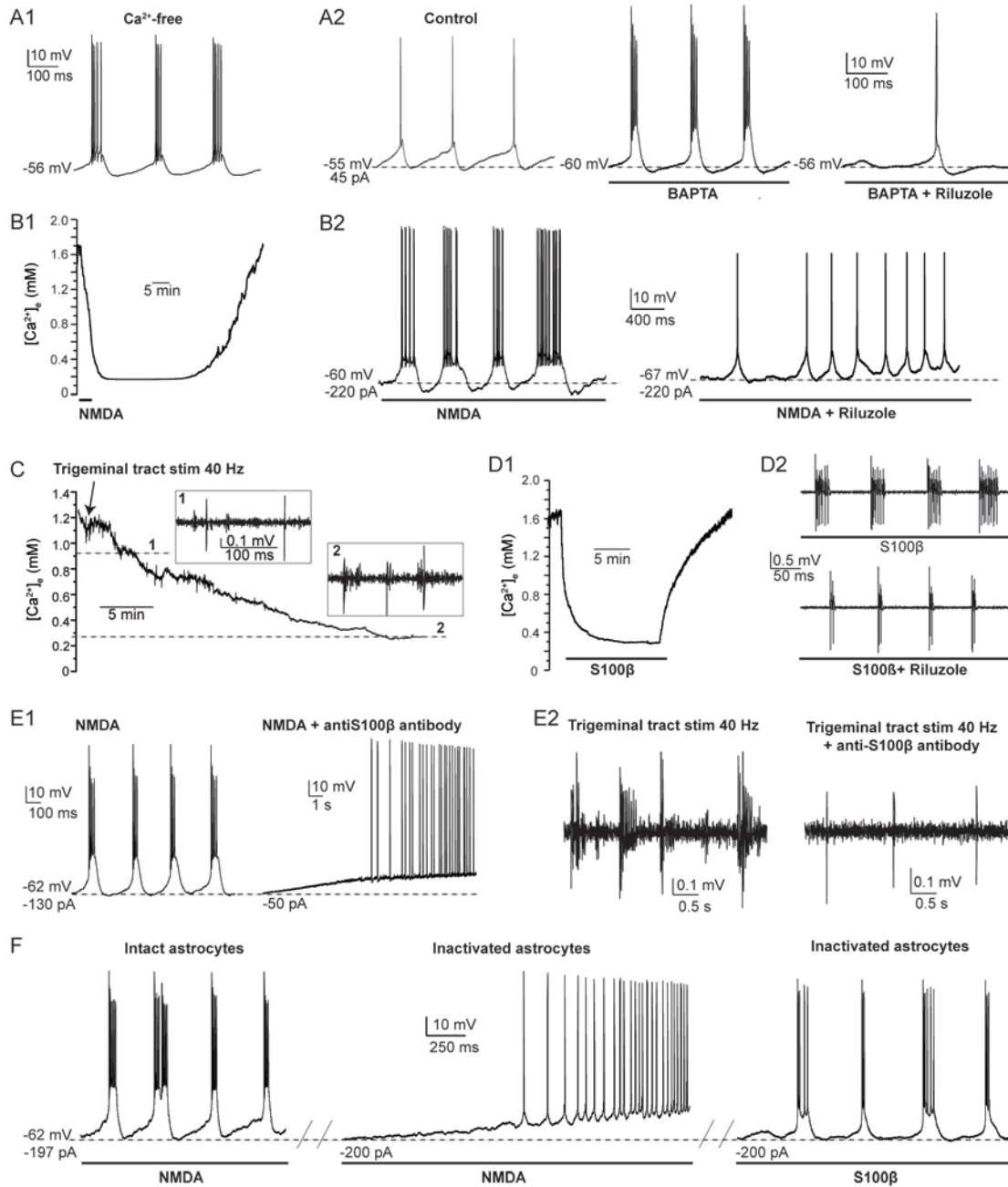
Figure 2. Involvement of astrocytes in the generation of bursts in the masticatory CPG. A1 , Neurons of the trigeminal main sensory nucleus (NVsnpr) display a bursting pattern in calcium-free medium. A2 , In control conditions, NVsnpr neurons fire tonically (left). Bath application of BAPTA causes one such neuron to burst (middle), and I_{NaP} channel blocker riluzole prevents the BAPTA-induced bursting in this neuron (right). B1 , Local application of NMDA leads to a significant decrease in extracellular calcium. B2 , NMDA-induced bursting in a NVsnpr neuron recorded in whole-cell configuration (left) is blocked by bath application of Riluzole (right). C , Electrical stimulation of the sensory trigeminal tract at 40 Hz also induces calcium depletion in the extracellular medium and bursts as seen in an extracellular recording of a NVsnpr neuron. Inset 1 shows a tonic discharge before calcium drops. Inset 2 shows a burst activity when extracellular calcium level is below 0.3 mM. D1 , The astrocytic protein S100 \beta causes extracellular calcium to diminish. D2 , A NVsnpr neuron discharges rhythmically in presence of S100 \beta (top) and S100 \beta -induced bursts are blocked by Riluzole (bottom). E1 , In whole-cell recordings, NMDA causes bursting (left) but not in presence of an antibody specifically directed against S100 \beta (right). E2 , In extracellular recordings, electrical stimulation of the sensory trigeminal tract at 40 Hz elicits bursting in control conditions (left) but not in presence of an anti-S100 \beta antibody (right). F , In whole-cell recordings, NMDA induced rhythmic bursting under control conditions (left), but only tonic firing after inactivating a neighboring astrocyte with intracellular dialysis of BAPTA (middle). Bursting was restored with an external application of S100 \beta (right).
