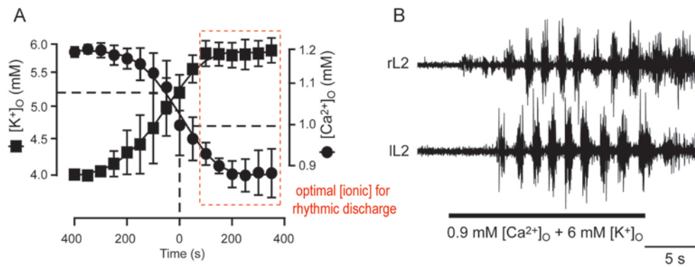
Figure 3. Example of synergistic interactions between potassium and calcium in rhythmogenesis. A , Evolution of extracellular concentration of calcium (circle) and potassium (square) before and after the onset (at 0 ms) of a locomotor-like bursting episode. Optimal concentrations of calcium and potassium for a bursting activity are emphasized by the dashed rectangle. A rhythmic activity appears at concentrations of calcium and potassium close to 0.9 and 6 mM, respectively. B , Extracellular recordings in the right and left L2 segments (rL2 and IL2) of rat spinal cord along with application of 0.9 mM [Ca^{2+}]_o and 6 mM [K^+]_o . Modified with permission from (19).
