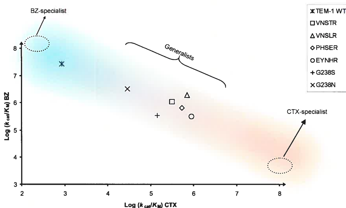
Figure 3.3 Comparison of catalytic efficiencies of wild-type TEM-1 \beta -lactamase with the mutants. Catalytic efficiencies are expressed as \text{Log}(k_{\text{cat}}/K_M) . The color gradient represents a hypothetical route starting from a specialized enzyme (BZ-specialist; blue) toward specialization for a new substrate (CTX-specialist; red). This shows the promiscuity of TEM-1. Generalized enzymes, such as mutants VNSTR, VNSLR, PHSER, EYNHR, G238S and G238N, are located in between. The wild-type TEM-1 enzyme is the most BZ-specialized, as evidenced by its high and low efficiencies toward BZ and CTX hydrolysis, respectively. The selected combinatorial mutants are generalized, although more efficient than G238N and G238S for hydrolysis of both substrates. EYNHR is the most CTX-specialized mutant. SWSSR is not represented because no kinetic assays with BZ have been performed on this mutant. Figure based on (52).
