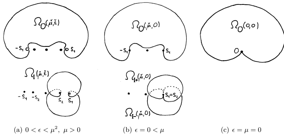
FIGURE 2.7. The domains \Omega_O(\check{\mu}, \check{\epsilon}) and \Omega_I(\check{\mu}, \check{\epsilon}) for selected values of \mu, \epsilon .
