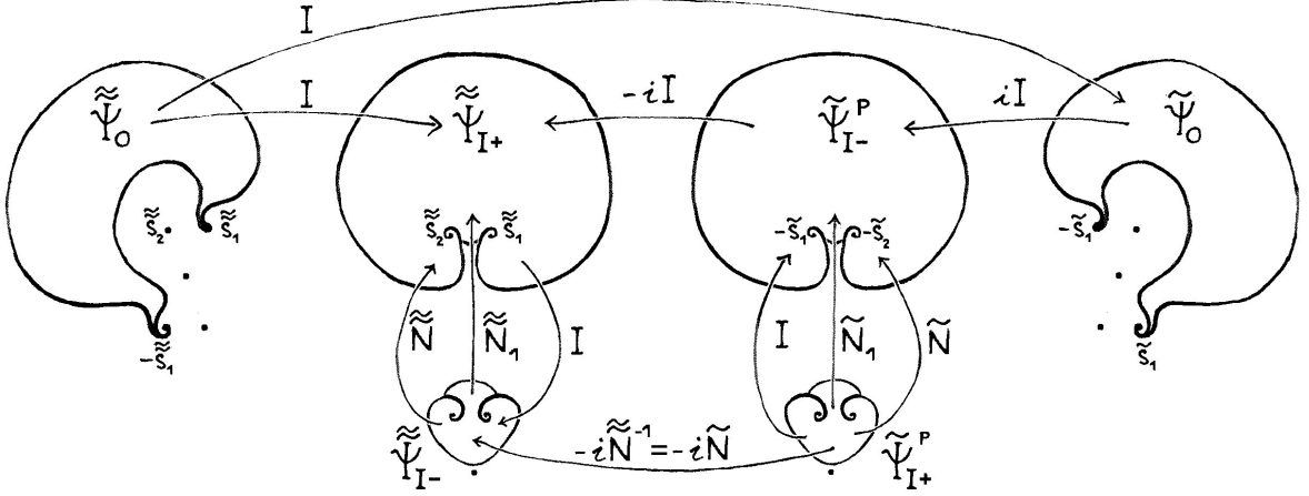
FIGURE 2.12. Connection matrices between fundamental solutions \Psi_\bullet of Lemma 2.3.12 with (\tilde{\mu}, \tilde{\epsilon}) = e^{2\pi i}(\mu, \epsilon) .
