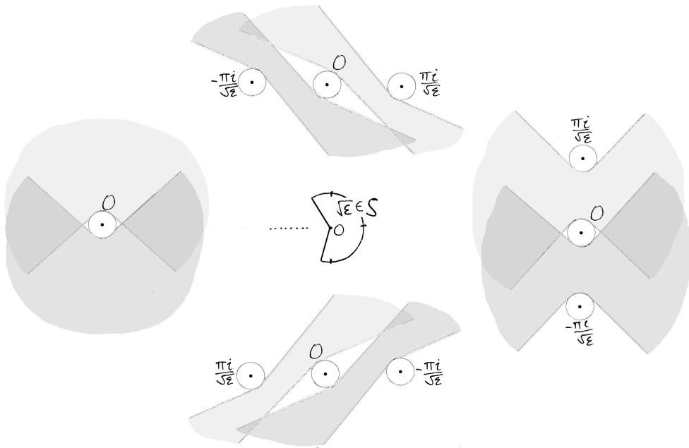
FIGURE 3.3. The domains Z(\sqrt{\epsilon}) of Theorem 3.2.4(i) in the time t -coordinate (3.4.1). They are obtained as unions of strips of convergence of the unfolded Laplace transforms \mathcal{L}_\alpha[\tilde{y}^+](x(t), \sqrt{\epsilon}) (3.5.21) with varying \alpha \in (\beta_1, \beta_2) \cap (\arg \sqrt{\epsilon} + \eta, \arg \sqrt{\epsilon} + \pi - \eta) (here \beta_1 \sim \frac{\pi}{4} , \beta_2 \sim \frac{3\pi}{4} ).
