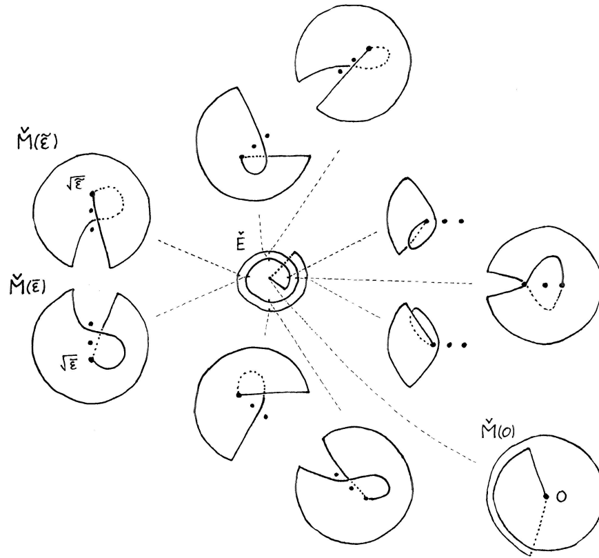
FIGURE 2.6. The ramified domains \check{M}(\check{\epsilon}) for the parameter \check{\mu} depending on \check{\epsilon} \in \check{\mathcal{E}} .
