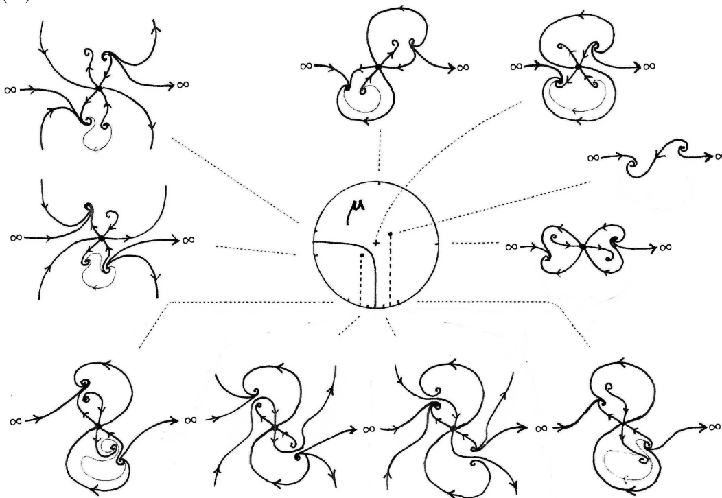
FIGURE 2.4. The real phase portrait of the vector field \chi according to \mu for selected values of \epsilon .
