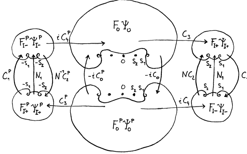
FIGURE 2.10. The connection matrices between the fundamental solutions F_{\bullet} \Psi_{\bullet} for a fixed parameter (\check{\mu}, \check{\epsilon}) , \check{\mu}^2 \neq \check{\epsilon} . For \check{\mu}^2 = \check{\epsilon} , only the fundamental solutions F_O \Psi_O and F_O^P \Psi_O^P persist, with the two corresponding connection matrices -iC_0, -iC_0^P . (Picture with (\check{\mu}, \check{\epsilon}) as in Figures 2.9 and 2.7(a)).
