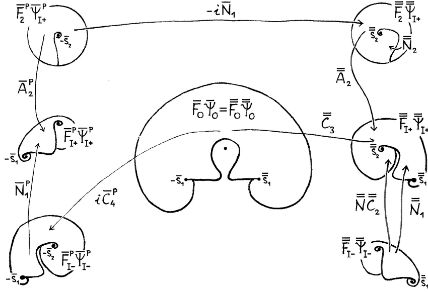
FIGURE 2.11. Connection matrices between fundamental solutions F_\bullet \Psi_\bullet of Lemma 2.3.12, with \check{\epsilon} fixed and \check{\mu} \neq \bar{\mu} . (Picture with \arg \check{\epsilon} = 0 .) The corresponding diagram for the diagonal solutions \Psi_\bullet of \bar{\Delta}^s is obtained by erasing all the F 's and replacing the matrices A_i, C_i by identity matrices. The top arrow in the diagram here \bar{F}_2^P \bar{\Psi}_{I+}^P \xrightarrow{-i\bar{N}_1} \bar{F}_2^P \bar{\Psi}_{I+}^P follows from the corresponding arrow \bar{\Psi}_{I+}^P \xrightarrow{-i\bar{N}_1} \bar{\Psi}_{I+}^P which one can easily read in the corresponding diagram for the diagonal solutions.
