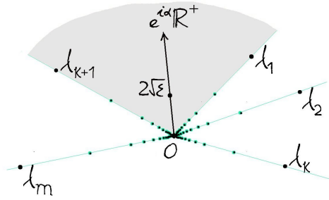
FIGURE 3.6. The resonant values of \sqrt{\epsilon} = \frac{\lambda}{2n} , \lambda \in \text{Spec } M(\epsilon) , n \in \mathbb{N}^* , accumulate along the rays \lambda\mathbb{R}^+ , dividing the \sqrt{\epsilon} -plane in sectors on which the local analytic solutions near x = \sqrt{\epsilon} \neq 0 converge as \sqrt{\epsilon} \rightarrow 0 to sectoral solutions.
