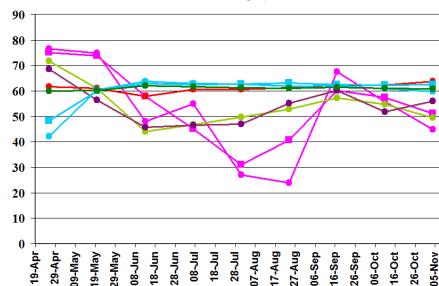
(K) \alpha_{s2}
