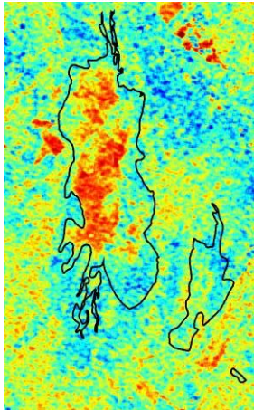
(F1) 2009-09-12, \lambda_{1N}
