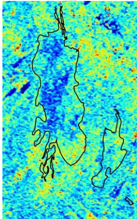
(E2) 2009-08-19, \lambda_{2N}
