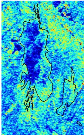
(F2) 2009-09-12, \lambda_{2N}
