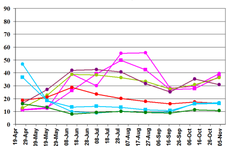
(I) \alpha_{s1}
