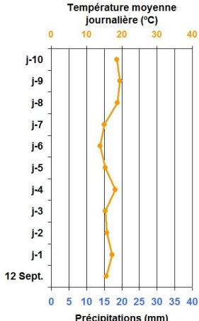
(F3) 2009-09-12
