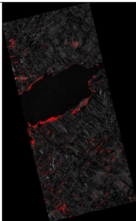
(A) \sigma_{hh}^0 / \sigma_{vv}^0 > 1.58
