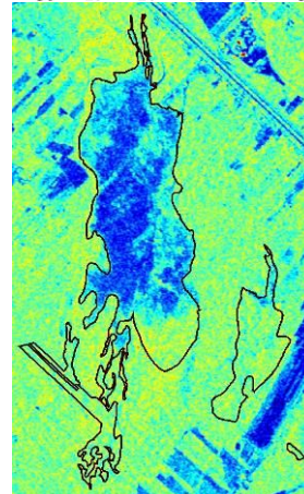
(F4) 2009-09-12, \sigma_{hv}^0
