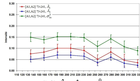
(D2) \lambda_2 , \lambda_3 et \sigma_{hv}^0
