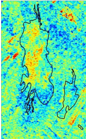
(E1) 2009-08-19, \lambda_{1N}
