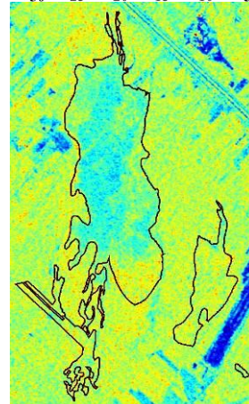
(E4) 2009-08-19, \sigma_{hv}^0
