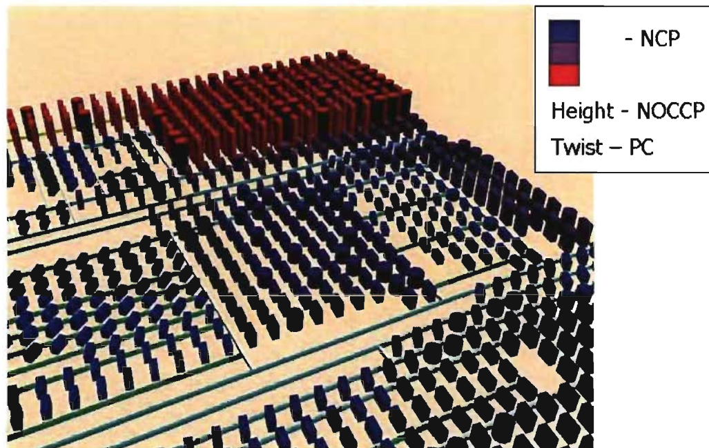
FIG. 4.11 – Occurrence de god package .
