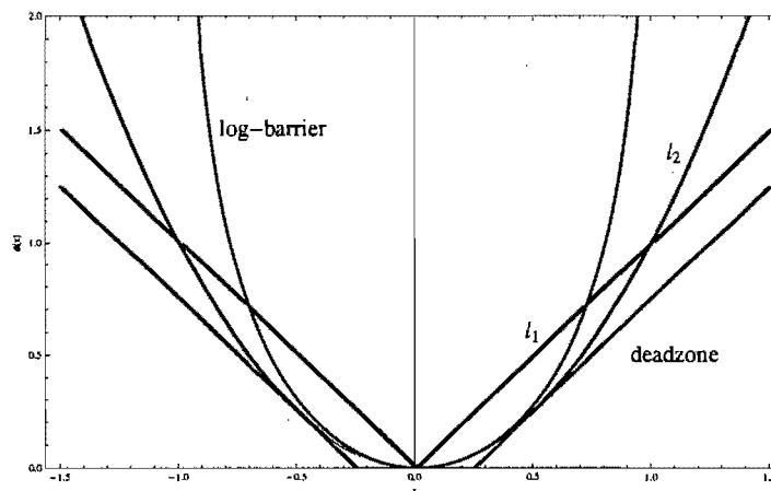
Figure 5.4. Norm functions
