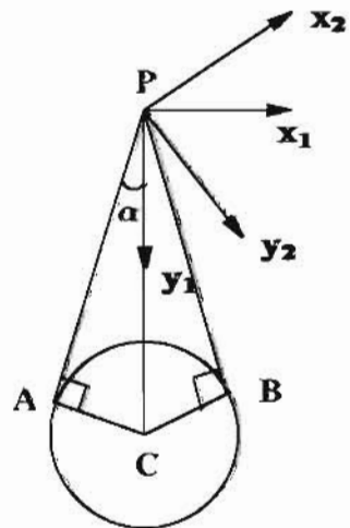
Figure 4.4. Two dimensional circle tangent problem.
