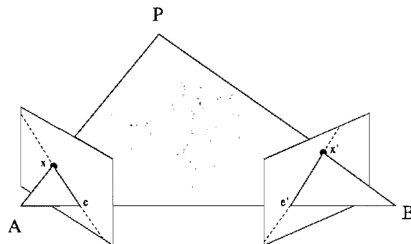
Figure 3.5. Epipolar geometry
