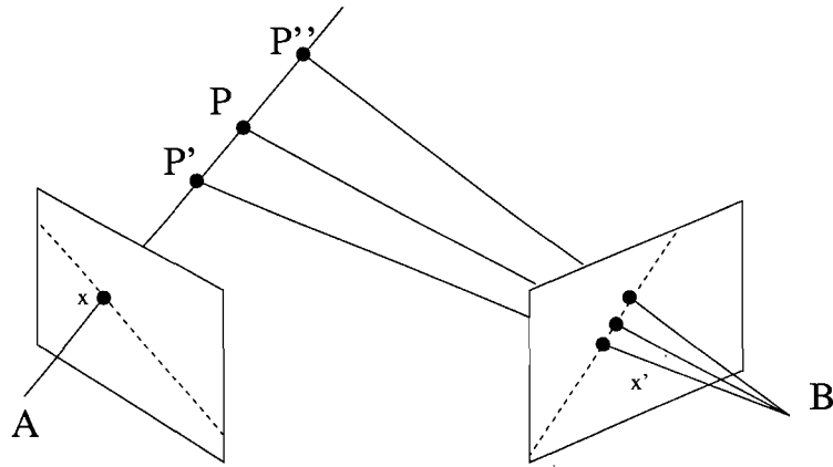
Figure 3.3. Triangulation
