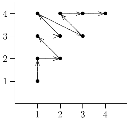
Figure 1: An ordering on \mathcal{S}[4] .
