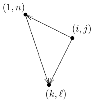
Figure 2: Proof of Theorem 3, case 1.
