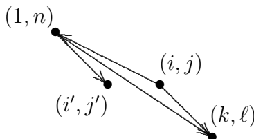
Figure 3: Proof of Theorem 3, case 2.
