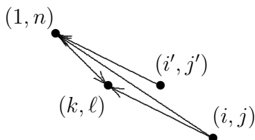
Figure 4: Proof of Theorem 3, case 3.
