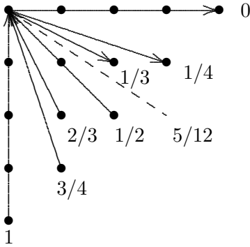
Figure 5: The quiver of the ordering \succeq_{5/12} on \mathcal{S}[5] .
