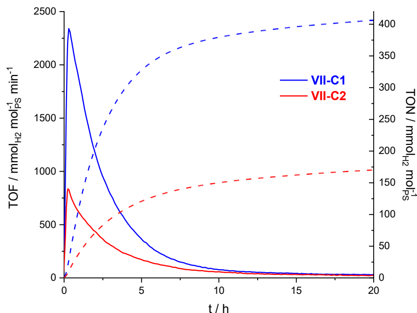
Figure VII-14. Hydrogen photoproduction with dinuclear complexes VII-C1 and VII-C2 as PS (0.1 mM) under blue light irradiation (LED centered at 445 nm); using [\text{Co}(\text{dmgH})_2(\text{py})\text{Cl}] as catalyst (1 mM), \text{dmgH}_2 (6 mM), TEOA as sacrificial electron donor (1 M) and \text{HBF}_4 as proton source (0.1 M) in DMF; TOF: solid lines; TON: dashed lines.
