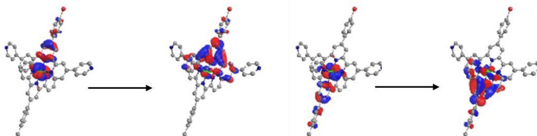
Figure IX-55. Natural transition analysis of the lowest singlet (left of arrow) to triplet (right of arrow) transition for complex III-C1 ; contributions of left transition 90%, contributions of right transition 6%.
