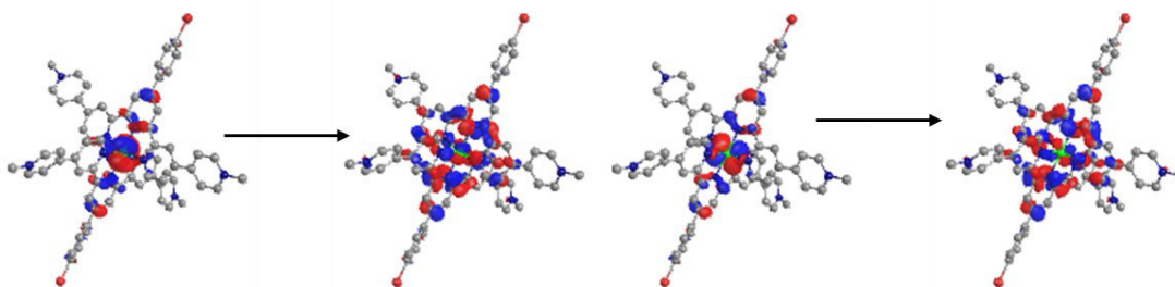
Figure IX-58. Natural transition analysis of the lowest singlet (left of arrow) to triplet (right of arrow) transition for complex V-C2 ; contributions of left transition 48%, contributions of right transition 48%.
