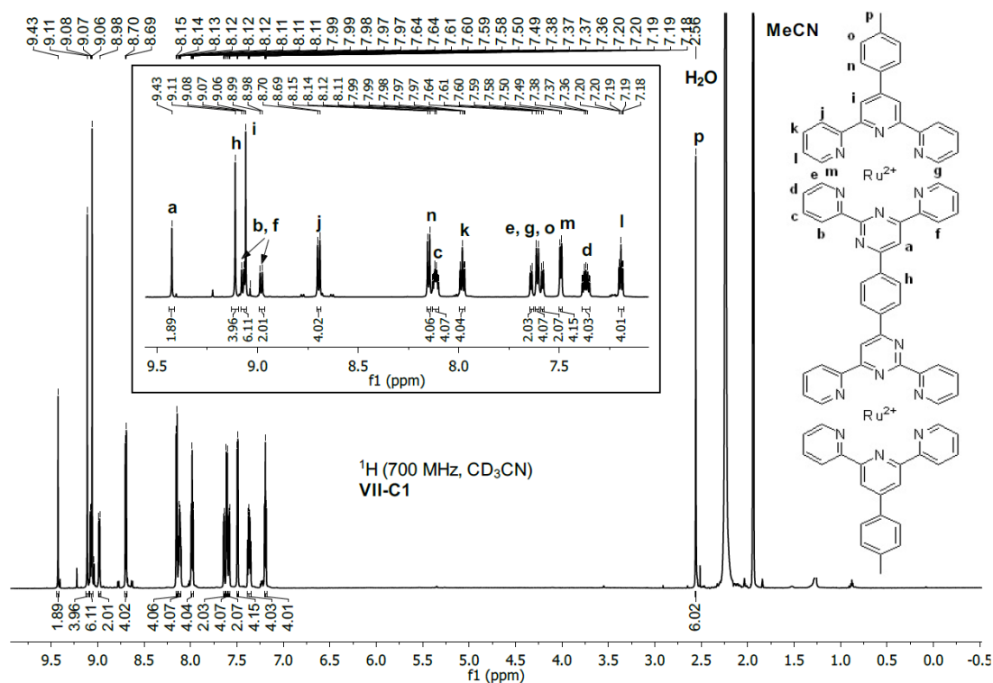
Figure IX-51. ^1\text{H} -NMR spectrum (700 MHz, \text{CD}_3\text{CN} ) of VII-C1.
