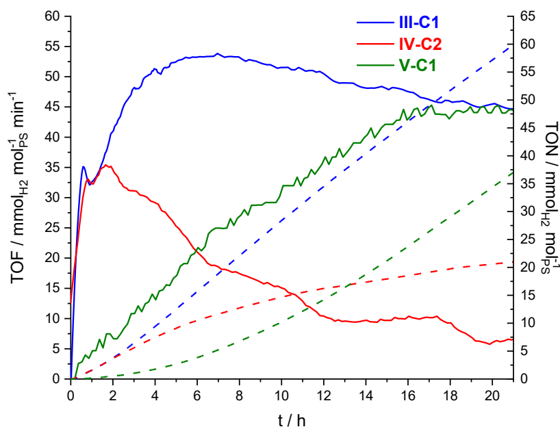
Figure V-7. Hydrogen photoproduction of complexes III-C1 , IV-C2 and V-C1 (0.1 mM) under blue light irradiation (LED centered at 445 nm); using K_2(PtCl_4) as pre-catalyst to form in-situ colloidal Pt (0.05 mM), TEOA as sacrificial electron donor (1 M) and HBf_4 as proton source (0.1 M) in DMF; TOF: solid lines; TON: dashed lines; adapted from Electrochemical and photophysical study of homoleptic and heteroleptic methylated ruthenium(II) bis-terpyridine complexes , Mira T. Rupp, Thomas Auvray, Garry S. Hanan, Dirk G. Kurth, European Journal of Inorganic Chemistry 2021 , 2021 (28), 2822-2829. Reproduced with permission of Wiley-VCH. [169]
