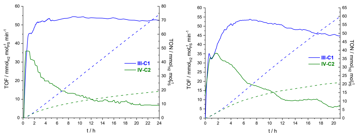
Figure IV-4. Hydrogen photoproduction with complexes III-C1 and IV-C2 as PS (0.1 mM) under blue light irradiation (LED centered at 445 nm); with TEOA as sacrificial electron donor (1 M) and \text{HBF}_4 as proton source (0.1 M) in DMF; left: [\text{Co}(\text{H}_2\text{O})_6](\text{BF}_4)_2 as pre-catalyst (1 mM), with \text{dmgH}_2 (6 mM); right: \text{K}_2(\text{PtCl}_4) as pre-catalyst to form in-situ colloidal Pt (0.05 mM); TOF: solid lines; TON: dashed lines; adapted from Electrochemical and photophysical study of homoleptic and heteroleptic methylated ruthenium(II) bis-terpyridine complexes , Mira T. Rupp, Thomas Auvray, Garry S. Hanan, Dirk G. Kurth, European Journal of Inorganic Chemistry 2021 , 2021 (28), 2822-2829. Reproduced with permission of Wiley-VCH. [169]
