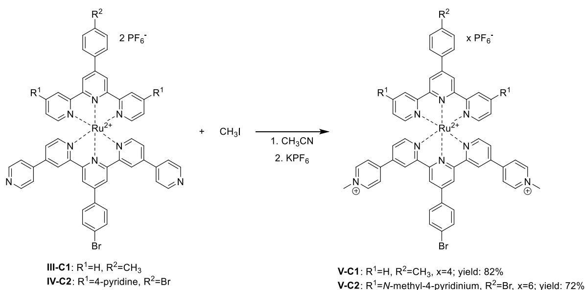
Scheme V-1. Synthesis of methylated complexes V-C1 and V-C2 .
