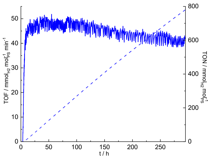
Figure III-6. Hydrogen photoproduction with complex III-C1 as PS (0.1 mM) under blue light irradiation (LED centered at 445 nm); with TEOA as sacrificial electron donor (1 M) and \text{HBF}_4 as proton source (0.1 M), [\text{Co}(\text{dmgH})(\text{dmgH}_2)\text{Cl}_2] as catalyst (1 mM), with \text{dmgH}_2 (6 mM) in DMF; TOF: solid line; TON: dashed line; adapted from Inorganic Chemistry , 2019 , 58 , 9127-9134. Reproduced with permission of American Chemical Society. [162]
