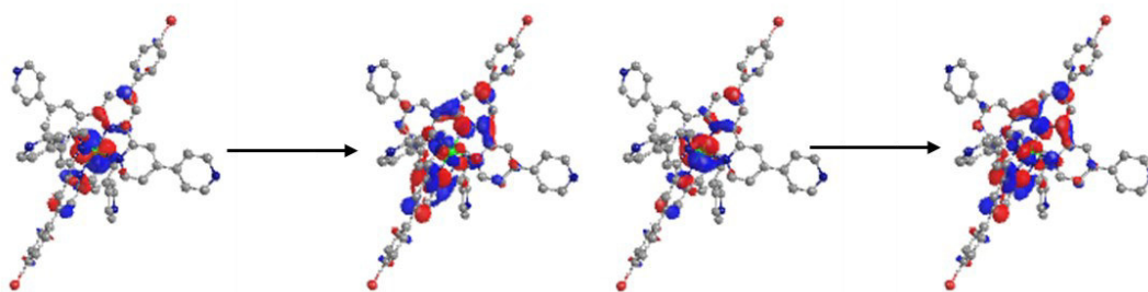
Figure IX-56. Natural transition analysis of the lowest singlet (left of arrow) to triplet (right of arrow) transition for complex IV-C2 ; contributions of left transition 48%, contributions of right transition 47%.
