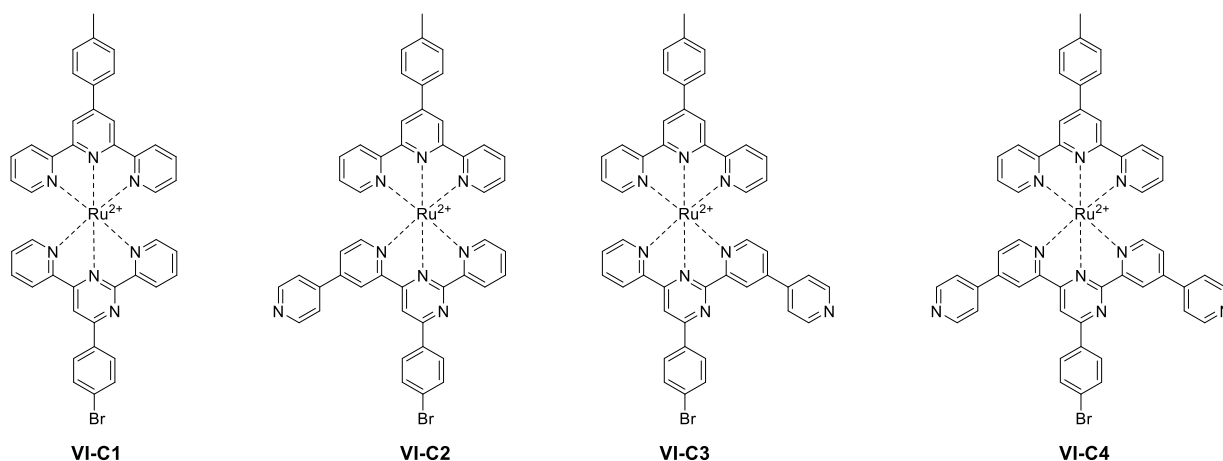
Chart VI-1. Structures of the pyrimidine containing complexes VI-C1 to VI-C4 ; the \text{PF}_6^- counterions are omitted for clarity.
