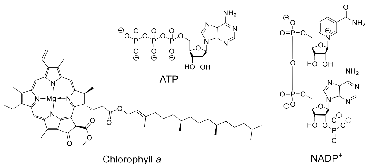
Chart I-1. Chemical structures of ATP, \text{NADP}^+ and chlorophyll a .
