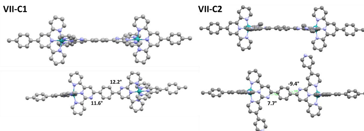
Figure VII-1. Optimized geometries of VII-C1 (left) and VII-C2 (right) with torsion angles between the pyrimidine rings and the phenyl spacer.
