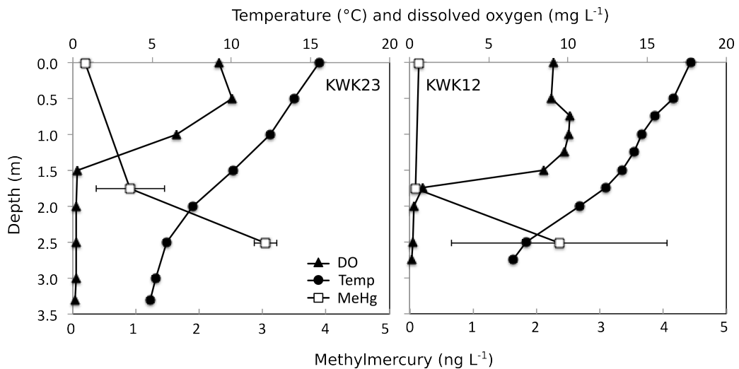
FIGURE S2. Vertical profiles of dissolved oxygen concentrations (DO, mg L -1 ), temperature (Temp, °C) and MeHg concentrations (ng L -1 ) for two stratified thermokarst ponds sampled near Kuujuarapik-Whapmagoostui in August 2009.
