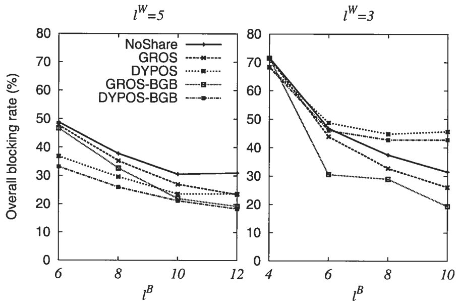
Figure 6.13: Overall blocking probabilities in LARGE-5.
