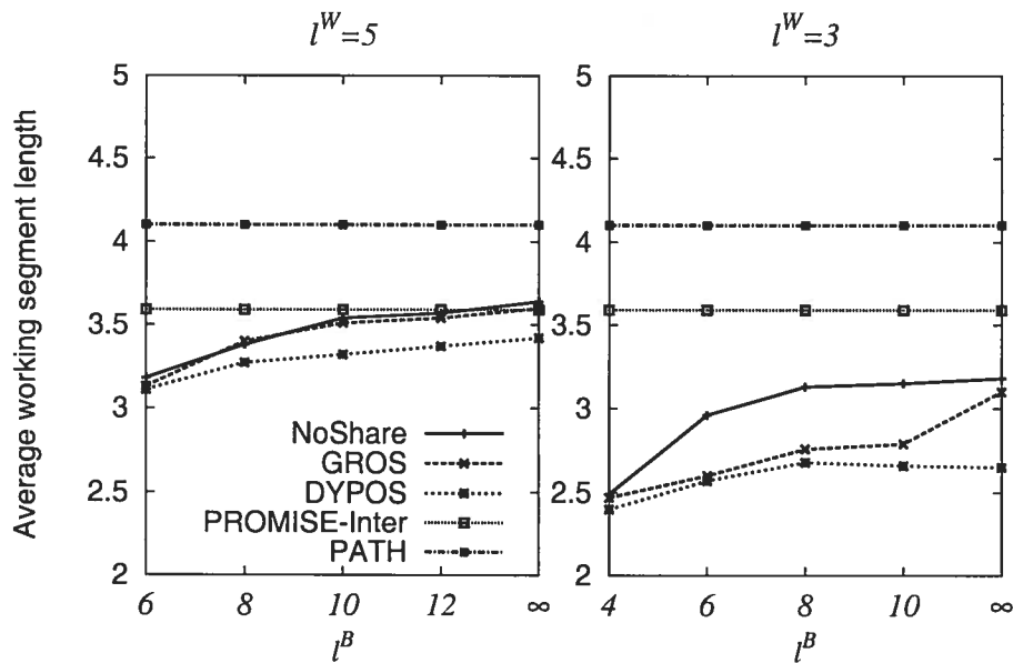
Figure 6.16: Average working segment lengths in LARGE-5
