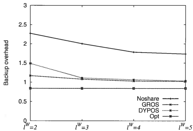
Figure 6.6: SMALL-5 network.
