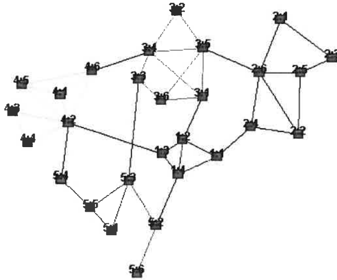
Figure 7.11: SMALL-5 network.
