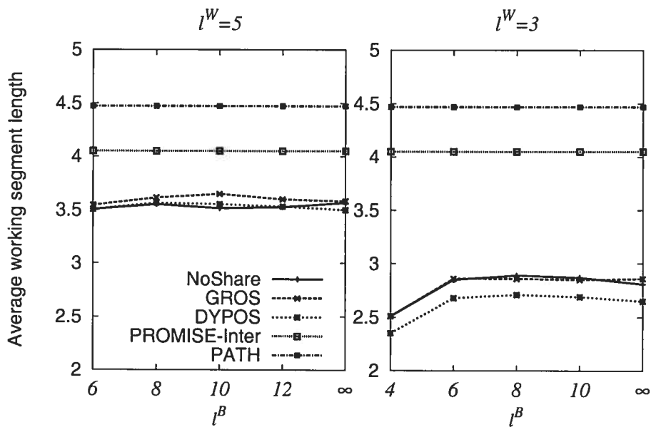
Figure 6.17: Average working segment lengths in LARGE-8
