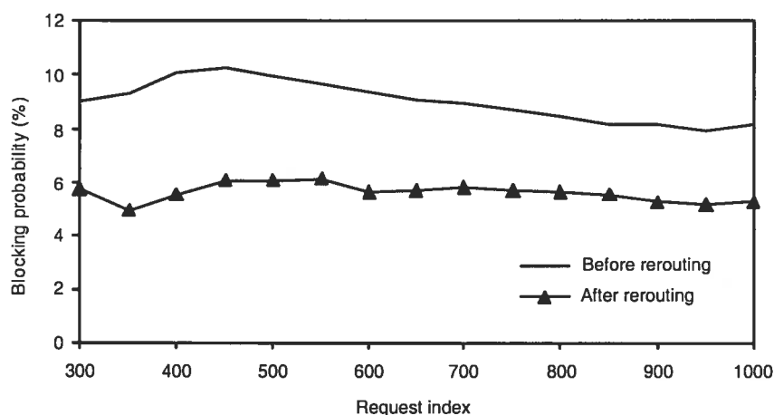
Figure 5.6: Blocking probability of WPF-RRLocal-Block before and after rerouting.
