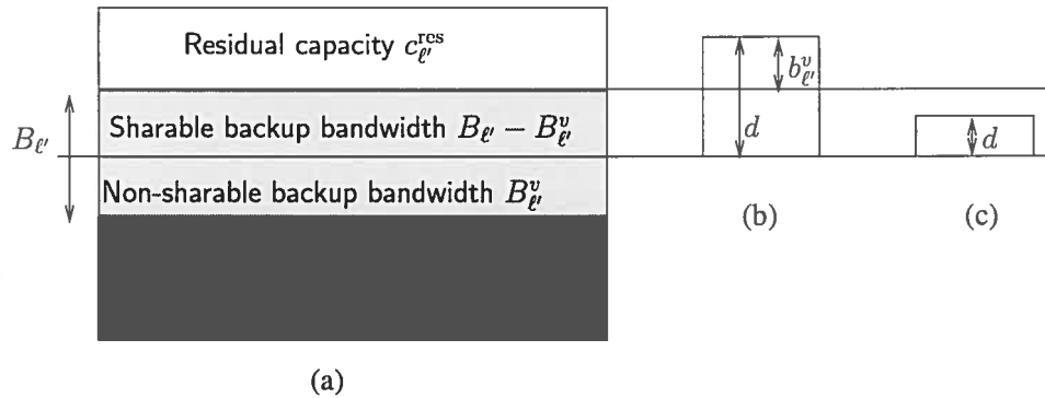
Figure 6.4: Bandwidth structure on a physical link \ell' (a) two examples of the required additional backup bandwidth on that link (b), (c).
