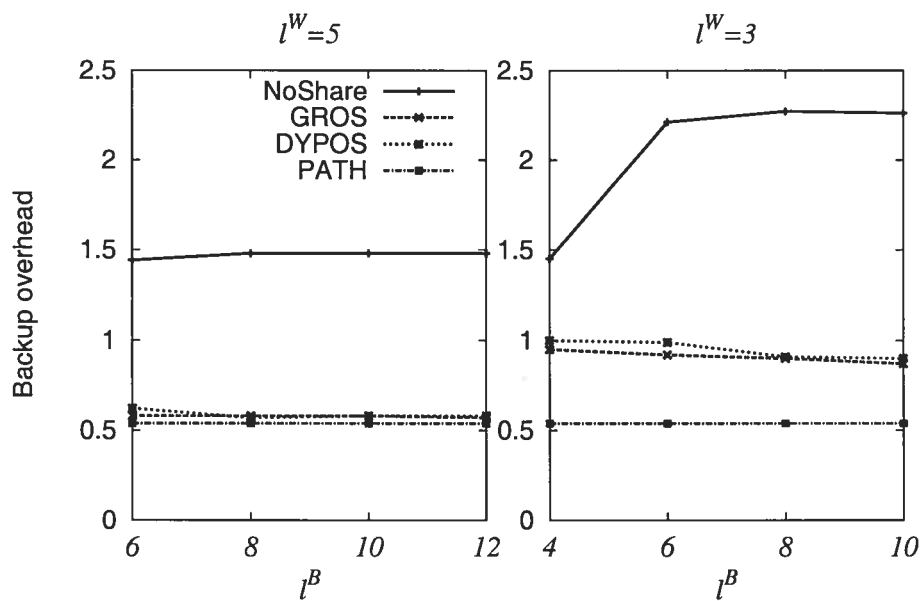
Figure 6.10: Backup overhead in LARGE-8.
