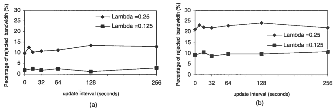
Figure 4.6: Bandwidth blocking probability of WPF at the inter-domain step (a) and Overall bandwidth blocking probability (b) under different update intervals.
