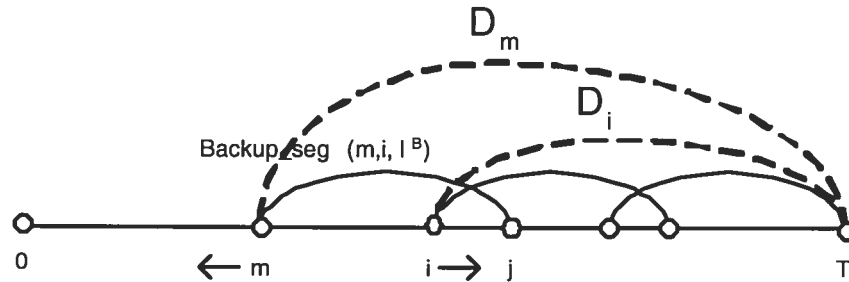
Figure 6.5: Working mechanism of the Dynamic programming algorithm
