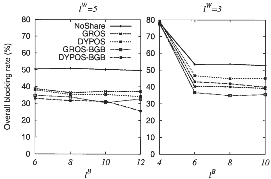
Figure 6.12: Overall blocking probabilities in LARGE-8.
