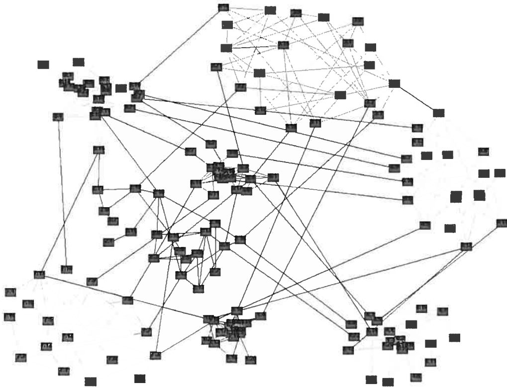
Figure 6.8: LARGE-8 network.
