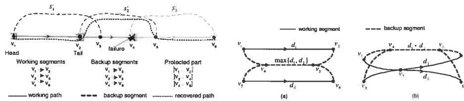
Figure 7.1: Example of Overlapping Segment Protection when v_4 fails. two backup segments can share The protected part [v_2..v_4] contains backup bandwidth (a) and cannot all links and nodes between v_2 exclusively and v_4 inclusively, thus v_4 is recovered using segment s_2' .
