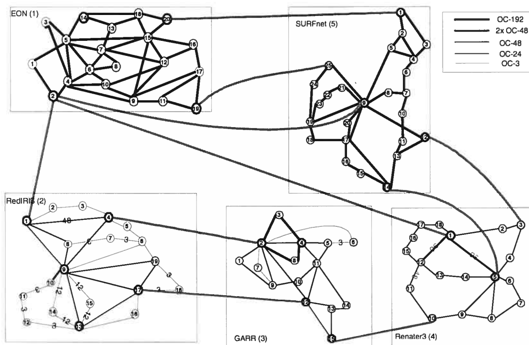
Figure 6.9: LARGE-5 network.
