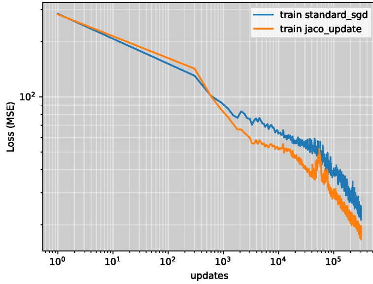
FIGURE 5.1. Training error for standard backpropagation (in blue) and updated backpropagation (in orange)
